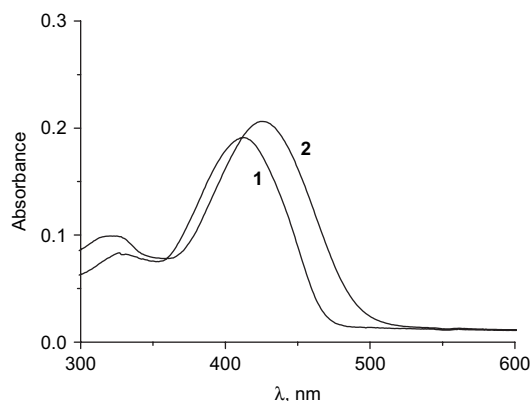
Figure 1. Absorption spectra of dyes 1 and 2 in ethanol. Selected data: [dye]= 2.5 \times 10^{-6} M, 1 : \lambda_{\text{max}}=413 nm ( \epsilon=6.9 \times 10^4 M -1 cm -1 ), 2 : \lambda_{\text{max}}=425 nm ( \epsilon=7.3 \times 10^4 M -1 cm -1 ).
